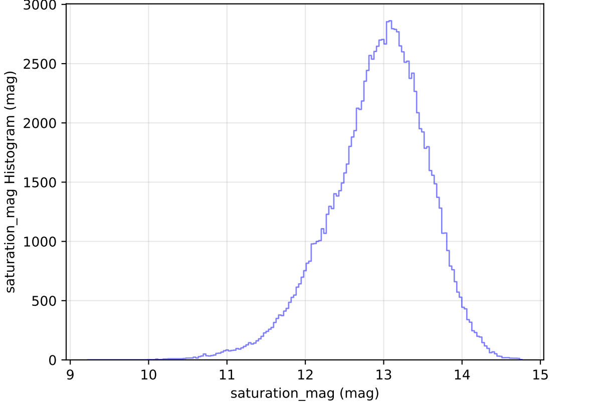
too_elab_r32_d3_giz_v3.4_10yrs All sky u band: saturation_mag Histogram
