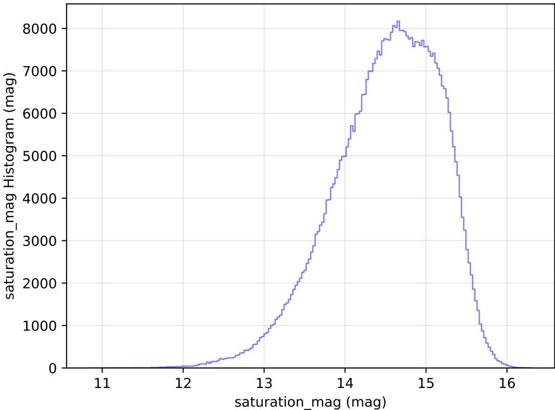
too_elab_r32_d3_giz_v3.4_10yrs All sky r band: saturation_mag Histogram
