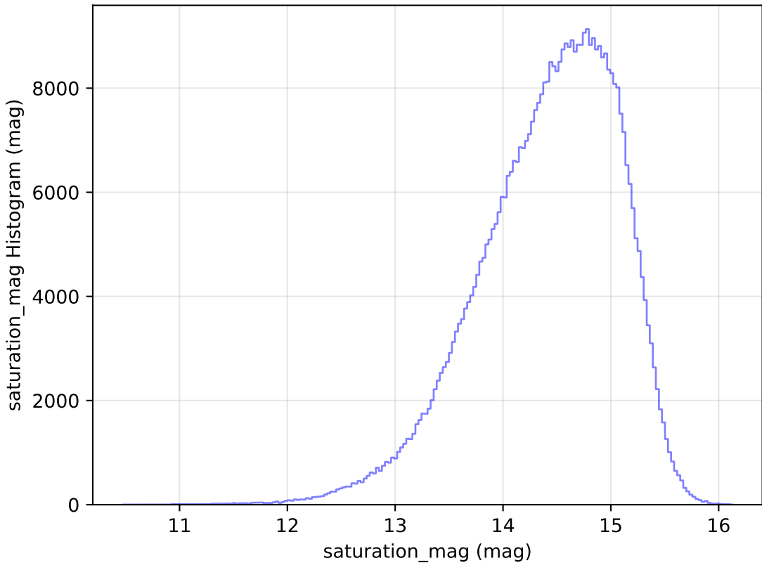
too_elab_r32_d3_giz_v3.4_10yrs All sky i band: saturation_mag Histogram
