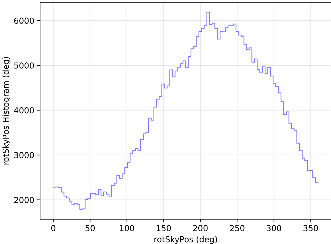
too_elab_r32_d3_giz_v3.4_10yrs WFD y band: rotSkyPos Histogram
