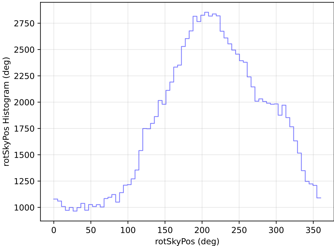
too_elab_r32_d3_giz_v3.4_10yrs WFD u band: rotSkyPos Histogram
