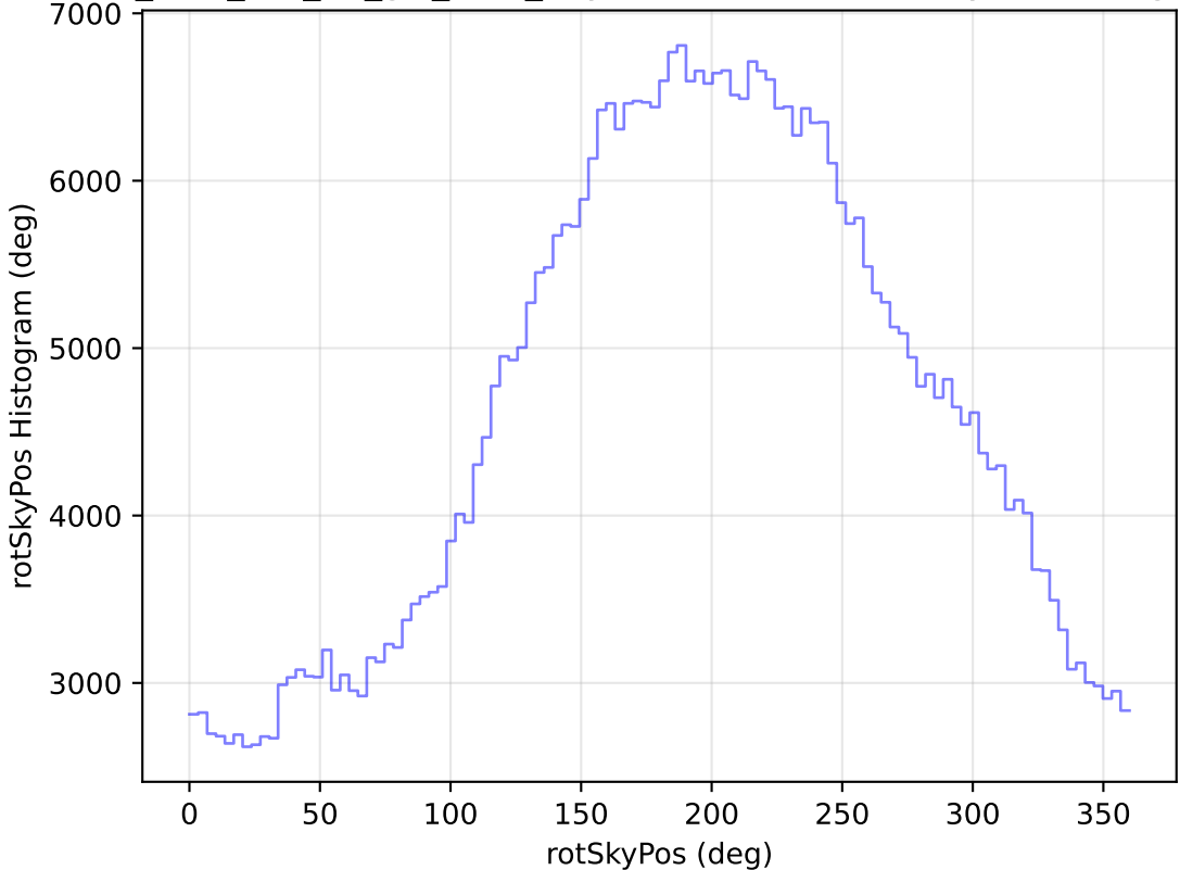
too_elab_r32_d3_giz_v3.4_10yrs WFD r band: rotSkyPos Histogram
