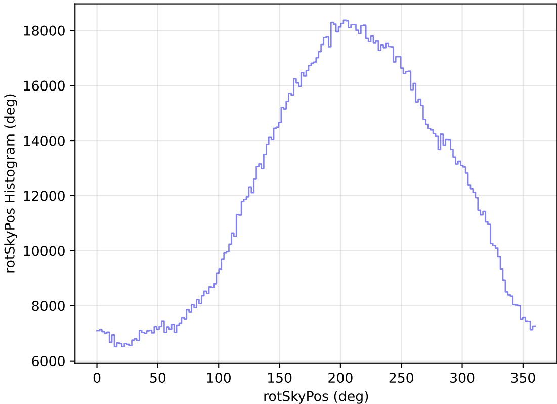
too_elab_r32_d3_giz_v3.4_10yrs WFD all bands: rotSkyPos Histogram
