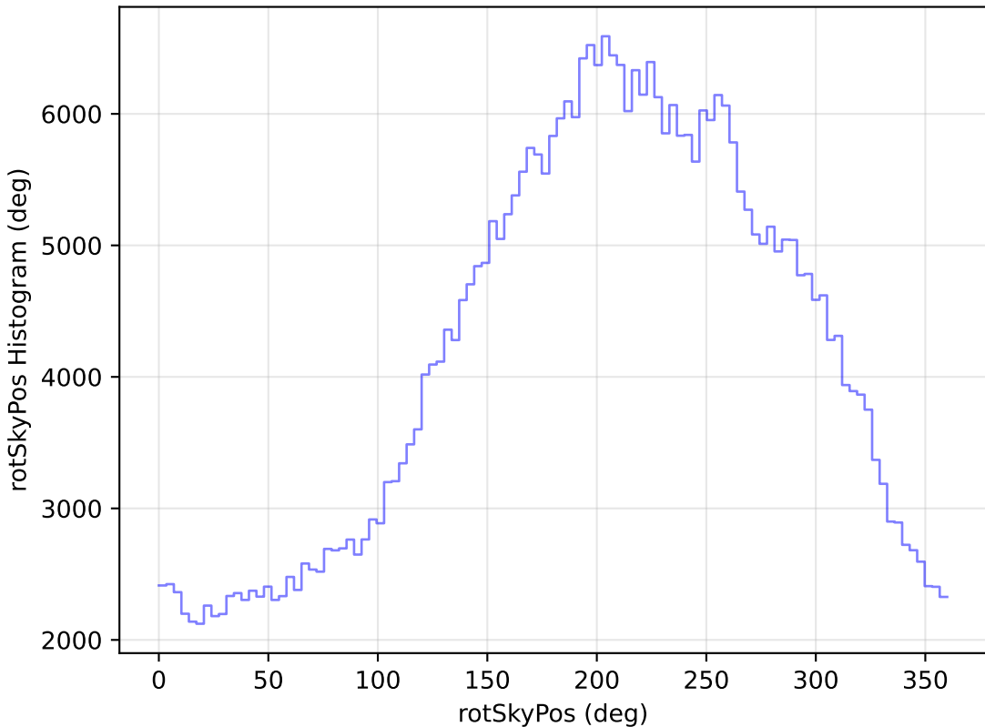
too_elab_r32_d3_giz_v3.4_10yrs All sky z band: rotSkyPos Histogram
