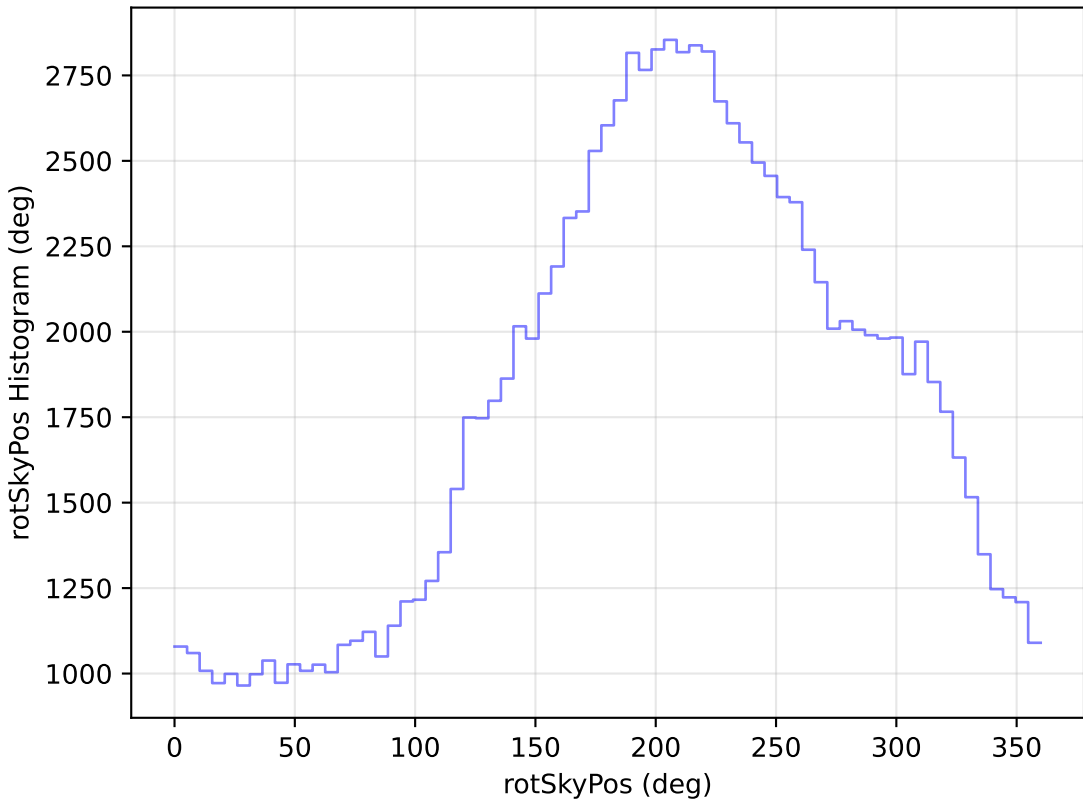
too_elab_r32_d3_giz_v3.4_10yrs All sky u band: rotSkyPos Histogram
