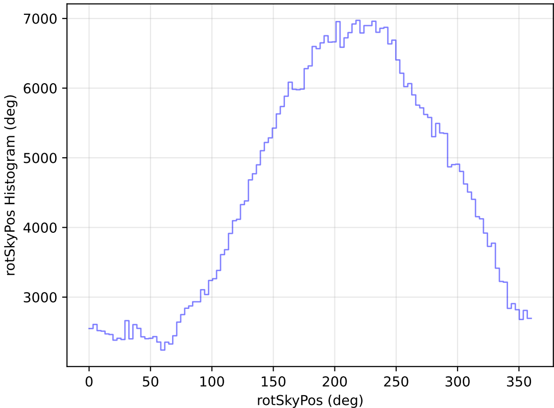
too_elab_r32_d3_giz_v3.4_10yrs All sky i band: rotSkyPos Histogram
