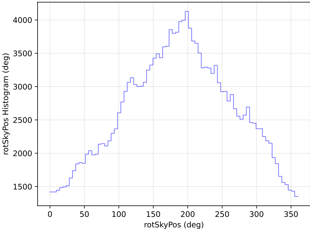
too_elab_r32_d3_giz_v3.4_10yrs All sky g band: rotSkyPos Histogram
