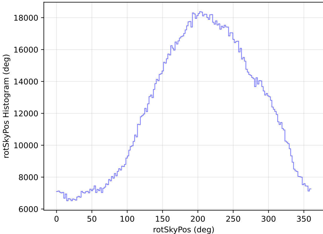
too_elab_r32_d3_giz_v3.4_10yrs All sky all bands: rotSkyPos Histogram
