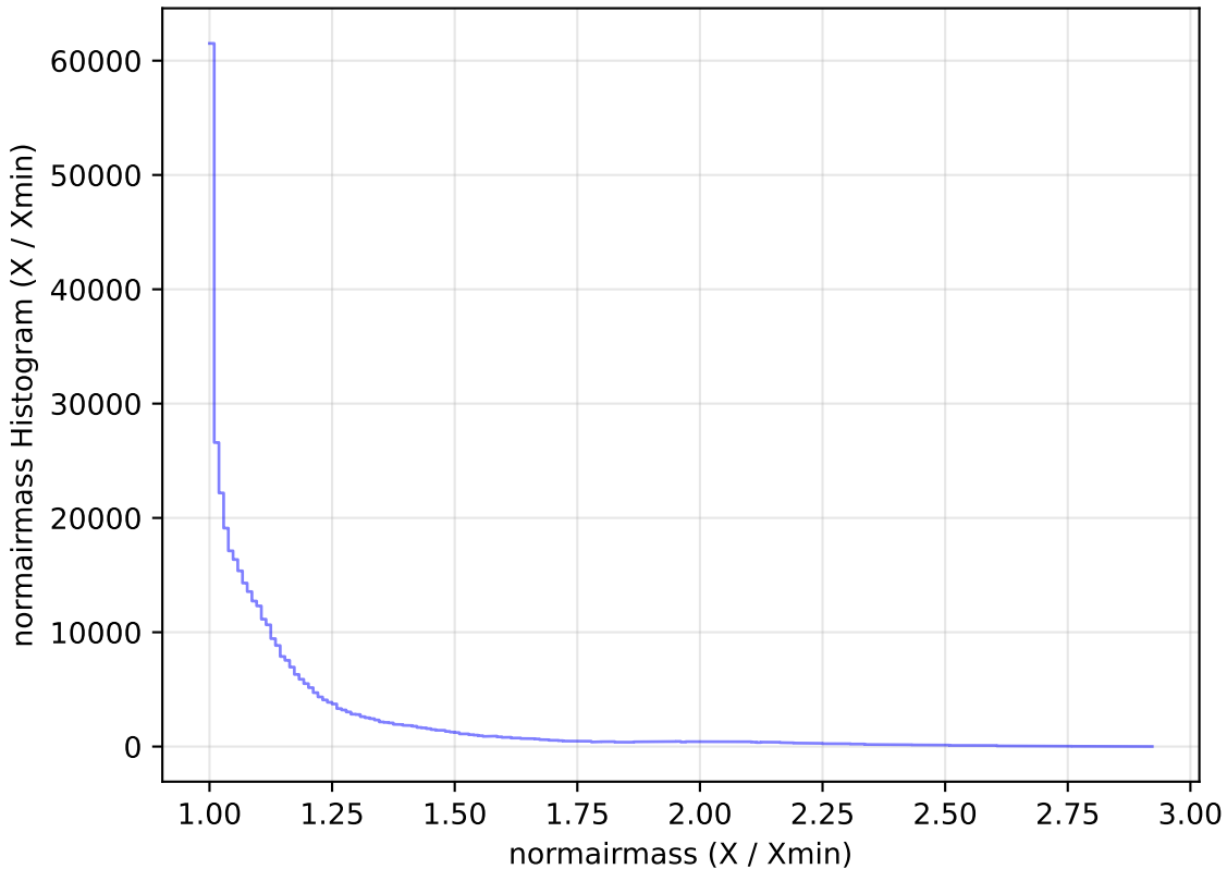
too_elab_r32_d3_giz_v3.4_10yrs WFD z band: normairmass Histogram
