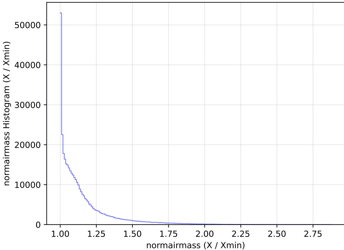
too_elab_r32_d3_giz_v3.4_10yrs WFD y band: normairmass Histogram
