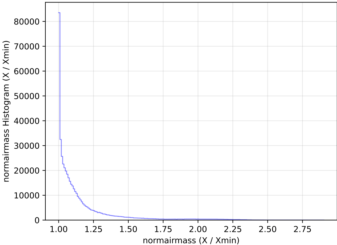
too_elab_r32_d3_giz_v3.4_10yrs WFD r band: normairmass Histogram
