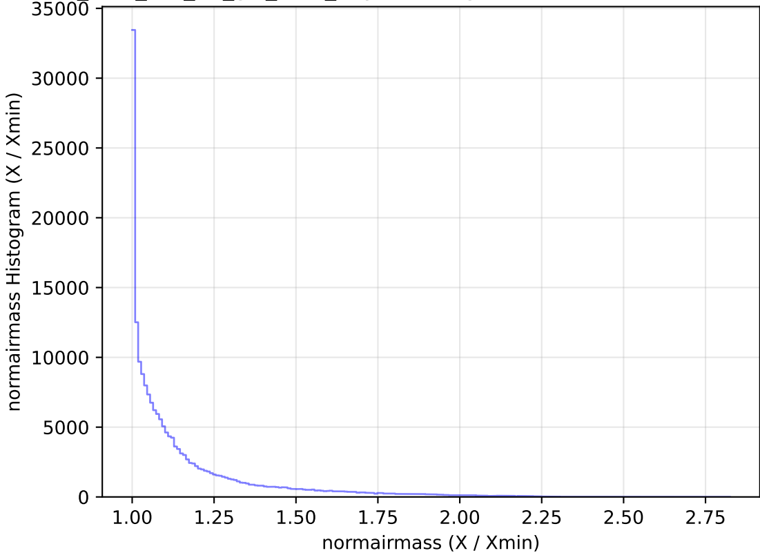
too_elab_r32_d3_giz_v3.4_10yrs WFD g band: normairmass Histogram
