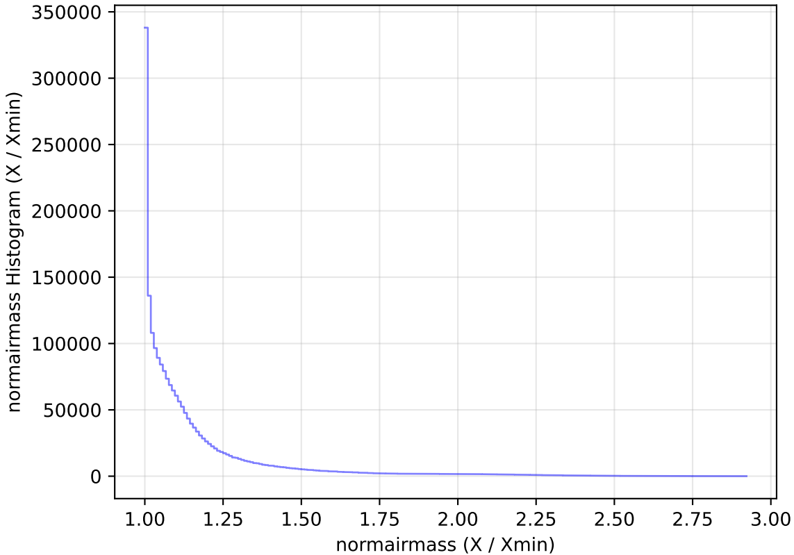
too_elab_r32_d3_giz_v3.4_10yrs WFD all bands: normairmass Histogram
