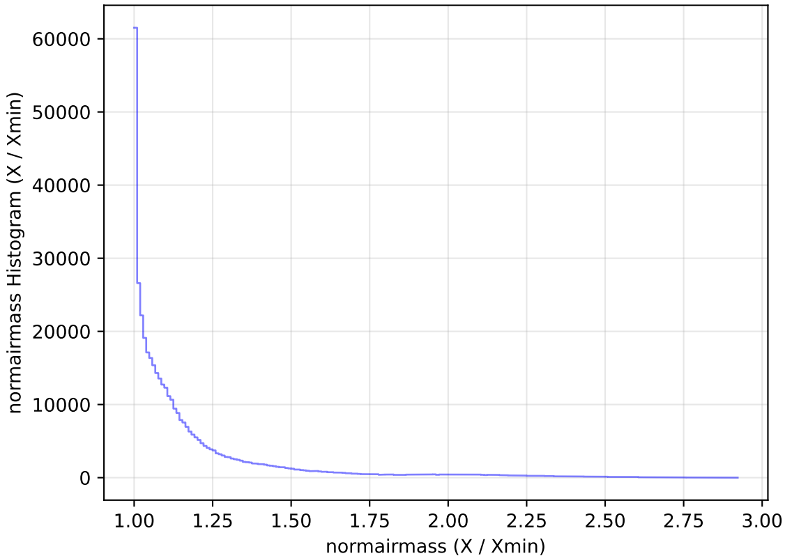
too_elab_r32_d3_giz_v3.4_10yrs All sky z band: normairmass Histogram
