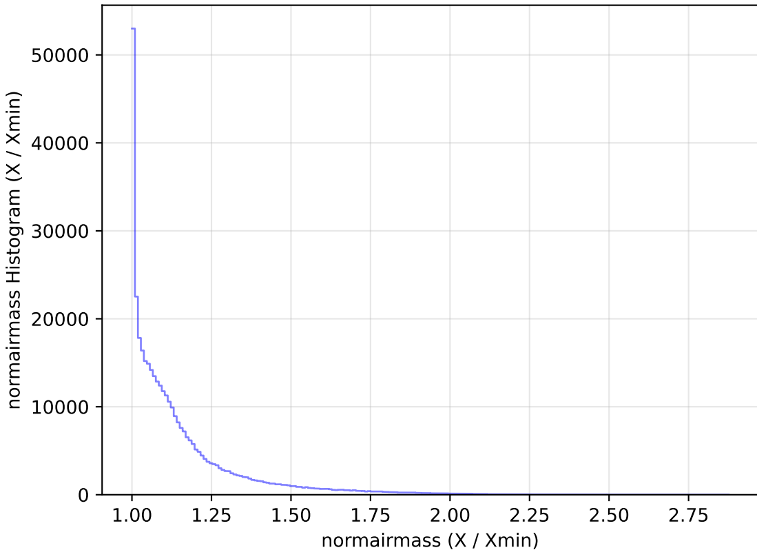
too_elab_r32_d3_giz_v3.4_10yrs All sky y band: normairmass Histogram
