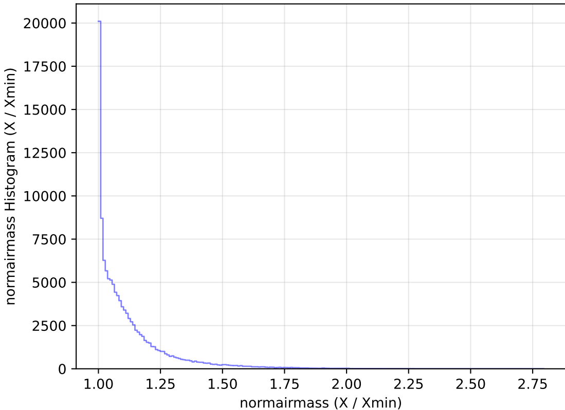
too_elab_r32_d3_giz_v3.4_10yrs All sky u band: normairmass Histogram
