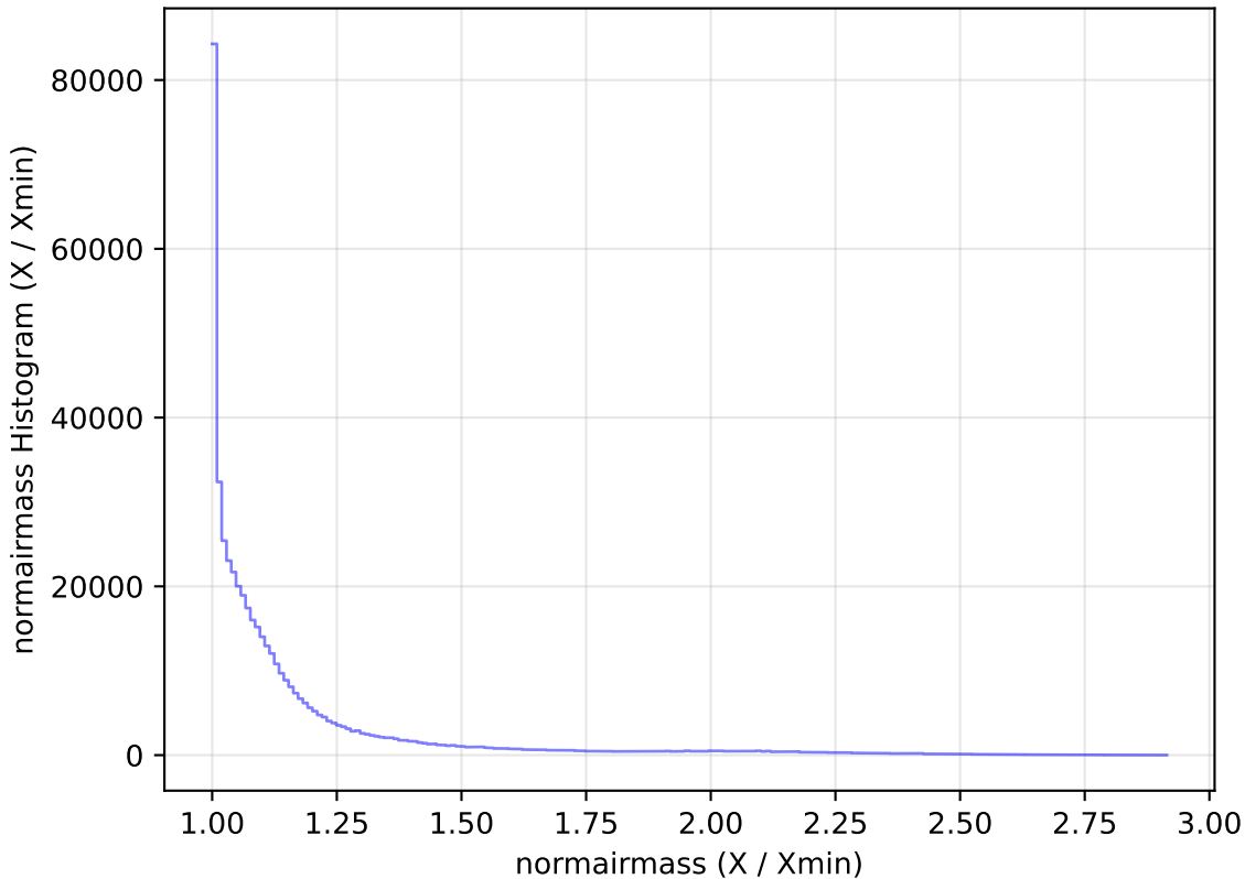
too_elab_r32_d3_giz_v3.4_10yrs All sky i band: normairmass Histogram
