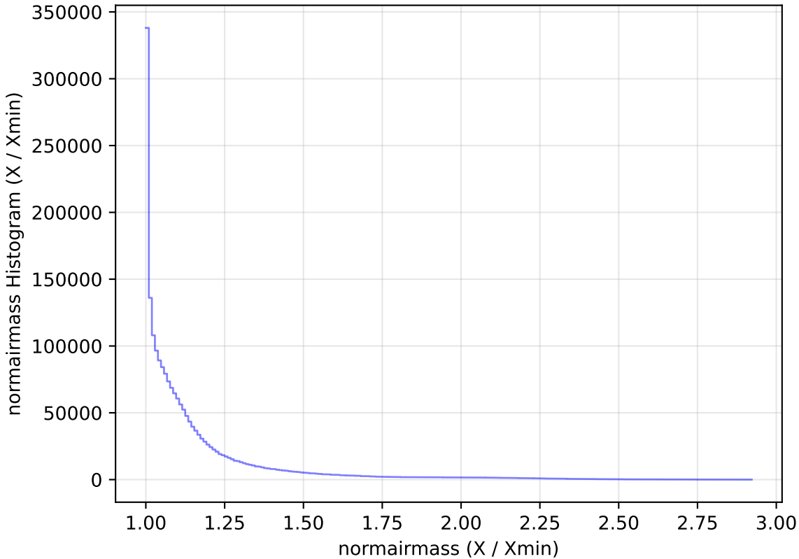
too_elab_r32_d3_giz_v3.4_10yrs All sky all bands: normairmass Histogram
