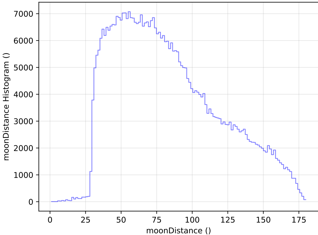
too_elab_r32_d3_giz_v3.4_10yrs WFD z band: moonDistance Histogram
