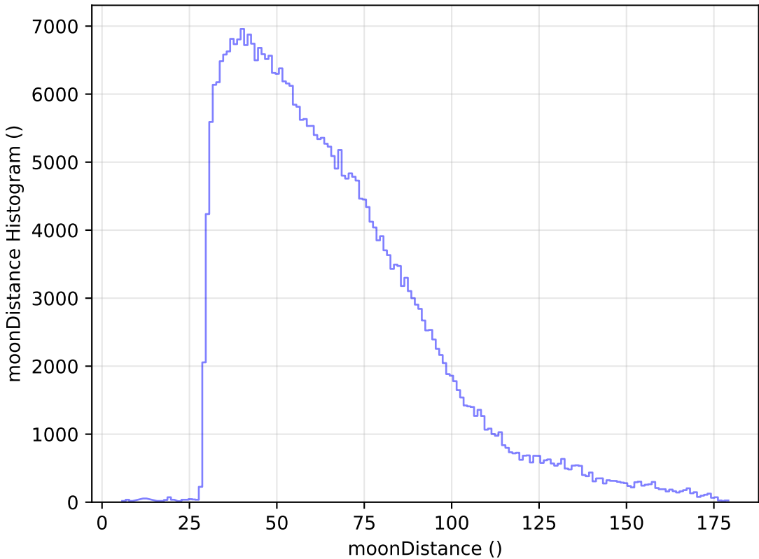
too_elab_r32_d3_giz_v3.4_10yrs WFD y band: moonDistance Histogram
