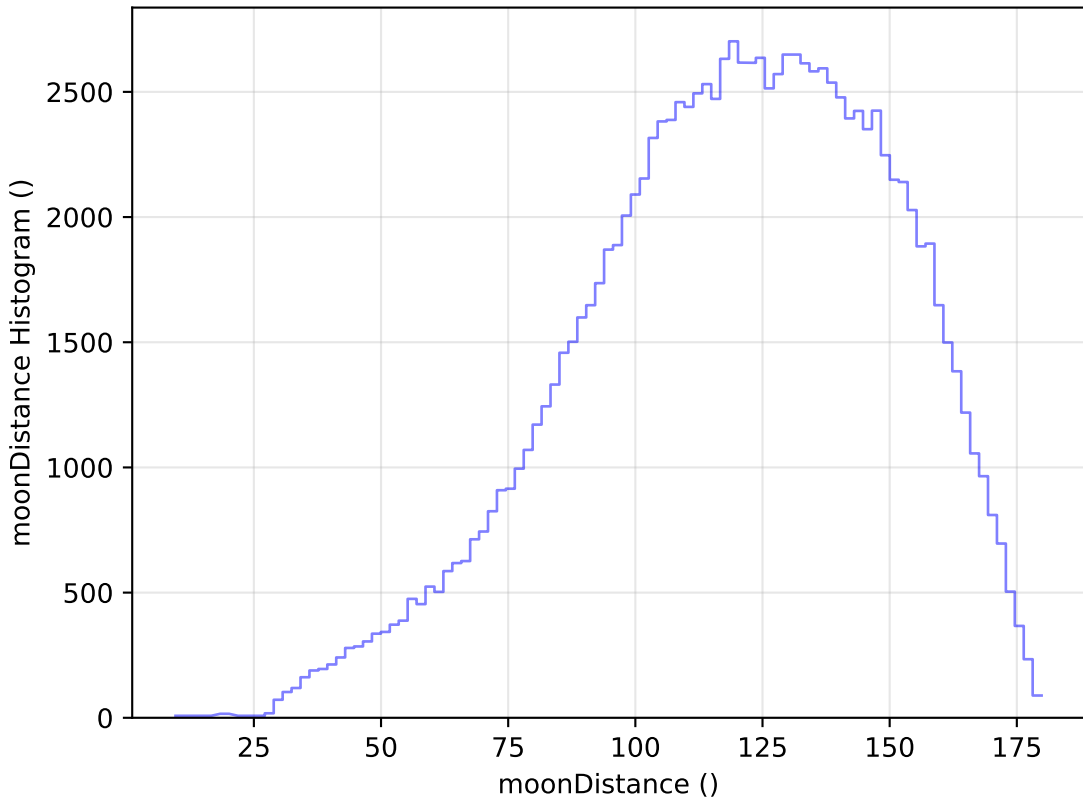
too_elab_r32_d3_giz_v3.4_10yrs WFD u band: moonDistance Histogram
