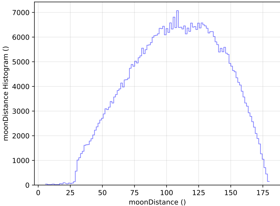
too_elab_r32_d3_giz_v3.4_10yrs WFD r band: moonDistance Histogram
