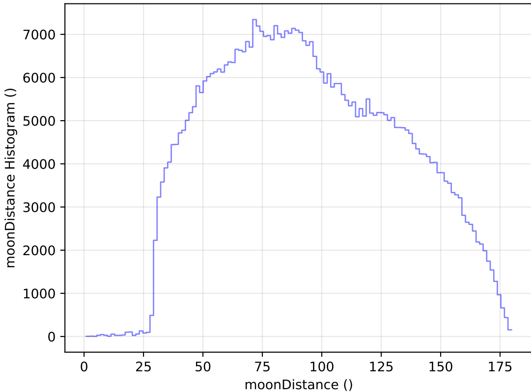
too_elab_r32_d3_giz_v3.4_10yrs WFD i band: moonDistance Histogram
