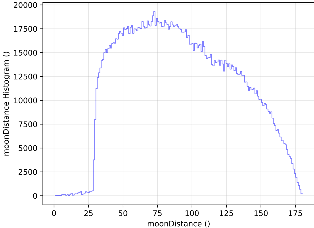
too_elab_r32_d3_giz_v3.4_10yrs WFD all bands: moonDistance Histogram
