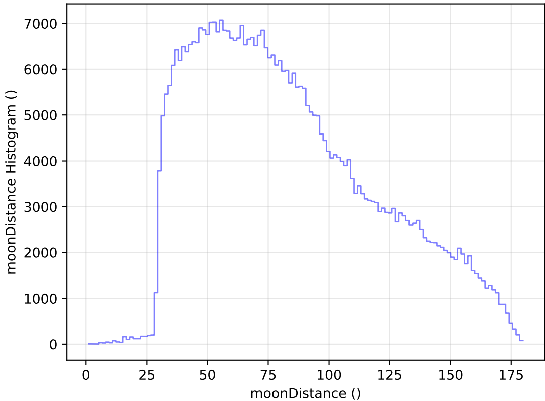
too_elab_r32_d3_giz_v3.4_10yrs All sky z band: moonDistance Histogram
