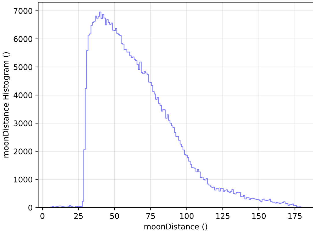
too_elab_r32_d3_giz_v3.4_10yrs All sky y band: moonDistance Histogram
