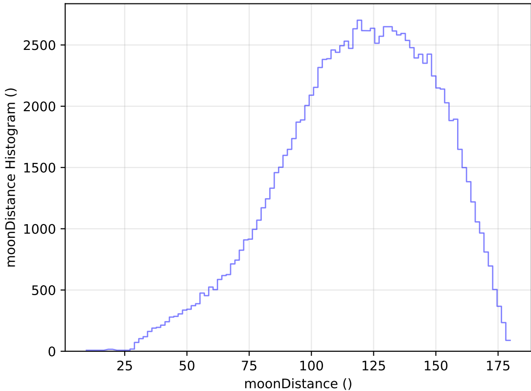
too_elab_r32_d3_giz_v3.4_10yrs All sky u band: moonDistance Histogram
