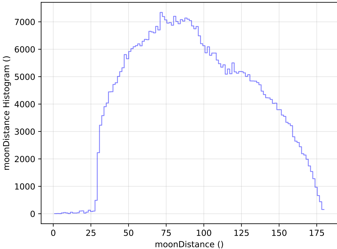
too_elab_r32_d3_giz_v3.4_10yrs All sky i band: moonDistance Histogram
