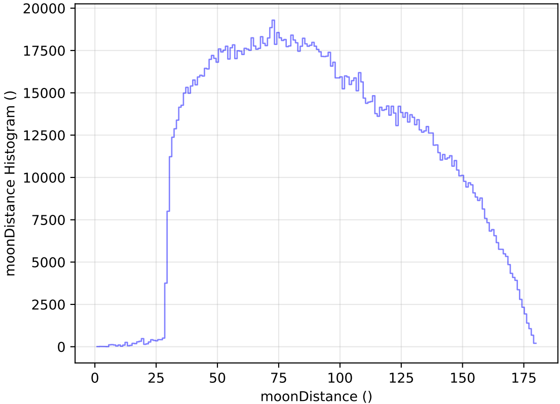
too_elab_r32_d3_giz_v3.4_10yrs All sky all bands: moonDistance Histogram
