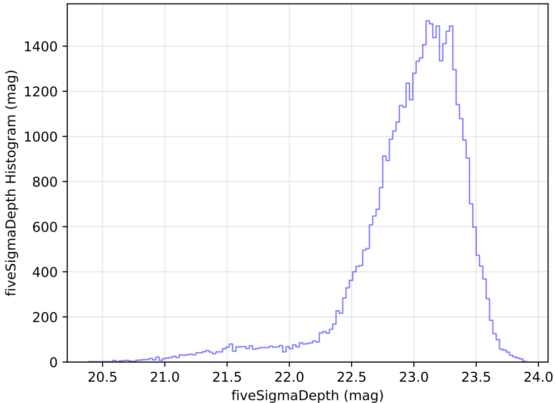
too_elab_r32_d3_giz_v3.4_10yrs Yr 1 z band: fiveSigmaDepth Histogram
