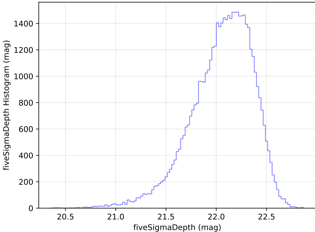
too_elab_r32_d3_giz_v3.4_10yrs Yr 1 y band: fiveSigmaDepth Histogram
