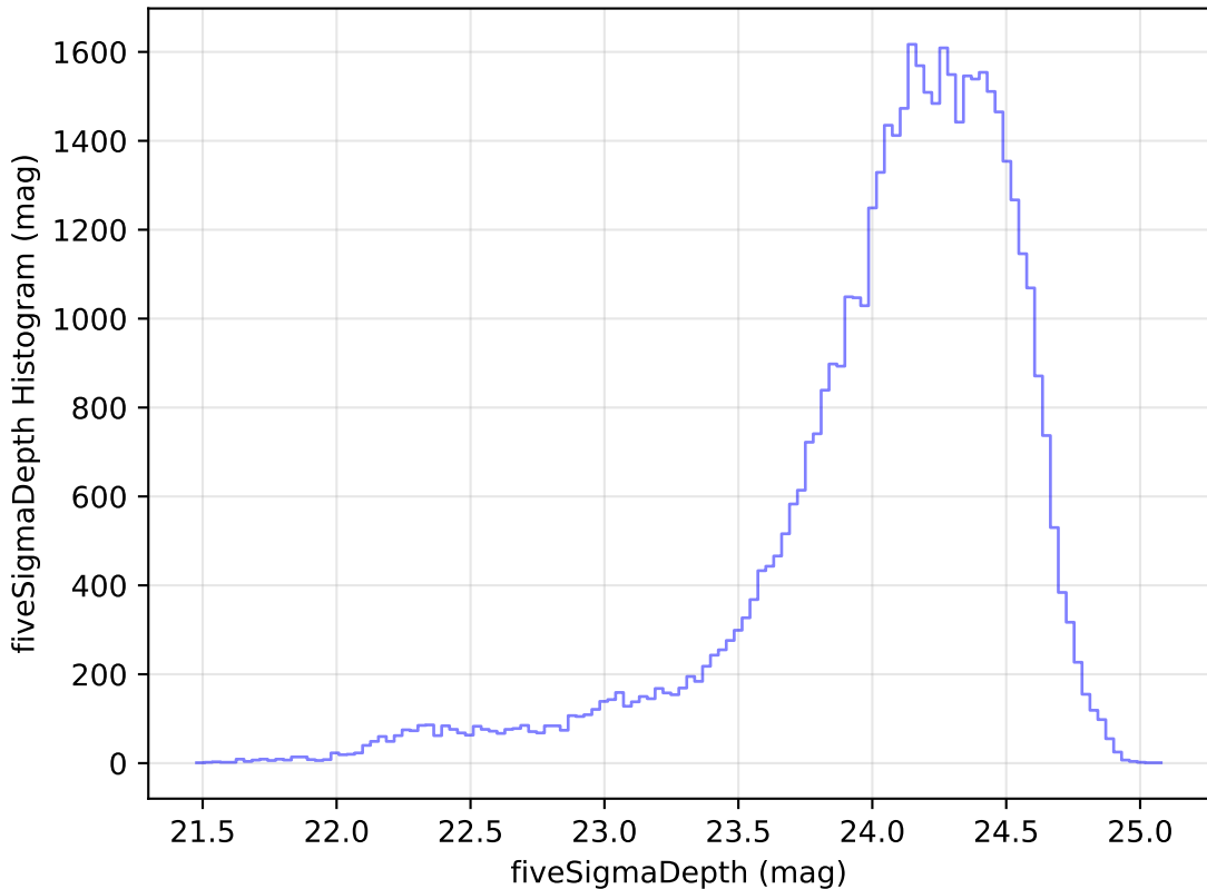
too_elab_r32_d3_giz_v3.4_10yrs Yr 1 r band: fiveSigmaDepth Histogram
