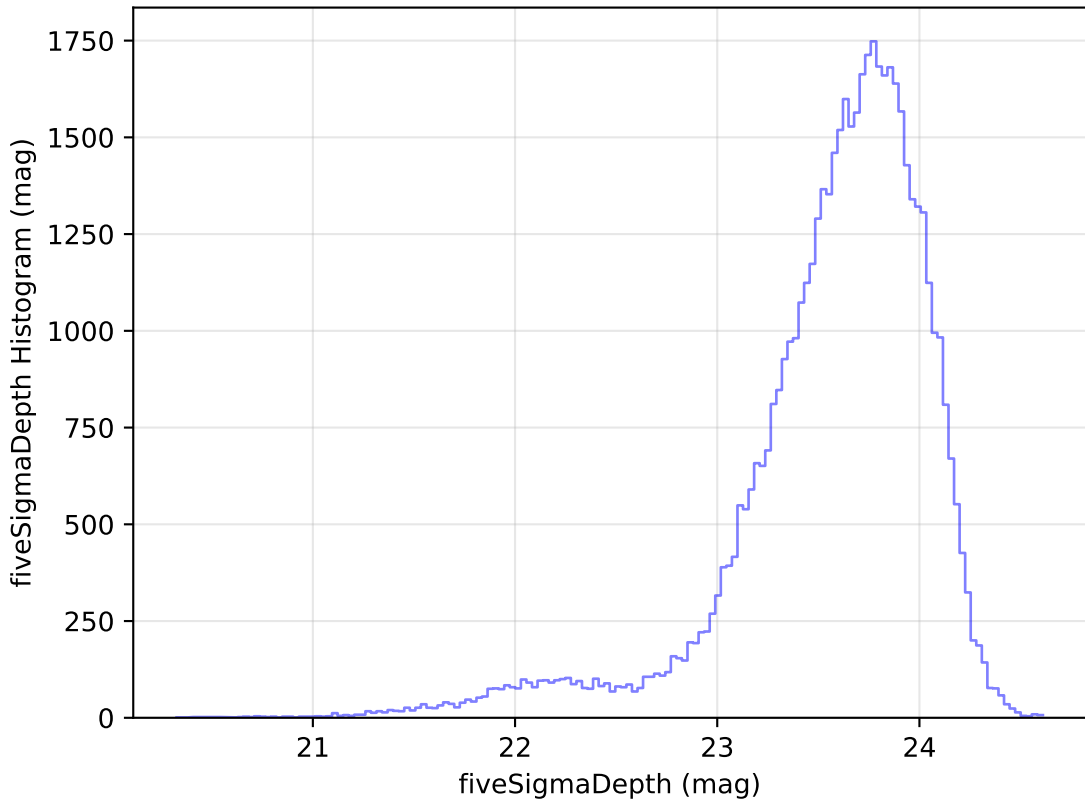
too_elab_r32_d3_giz_v3.4_10yrs Yr 1 i band: fiveSigmaDepth Histogram
