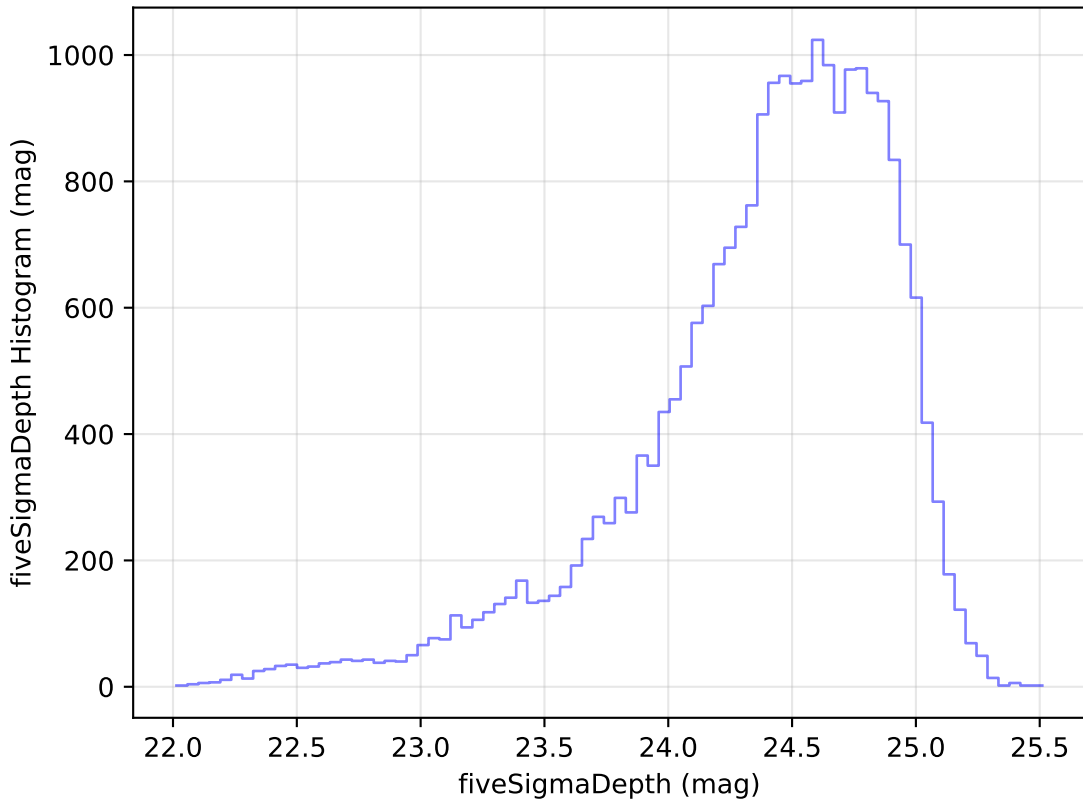
too_elab_r32_d3_giz_v3.4_10yrs Yr 1 g band: fiveSigmaDepth Histogram
