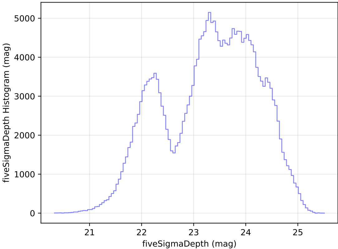
too_elab_r32_d3_giz_v3.4_10yrs Yr 1 all bands: fiveSigmaDepth Histogram
