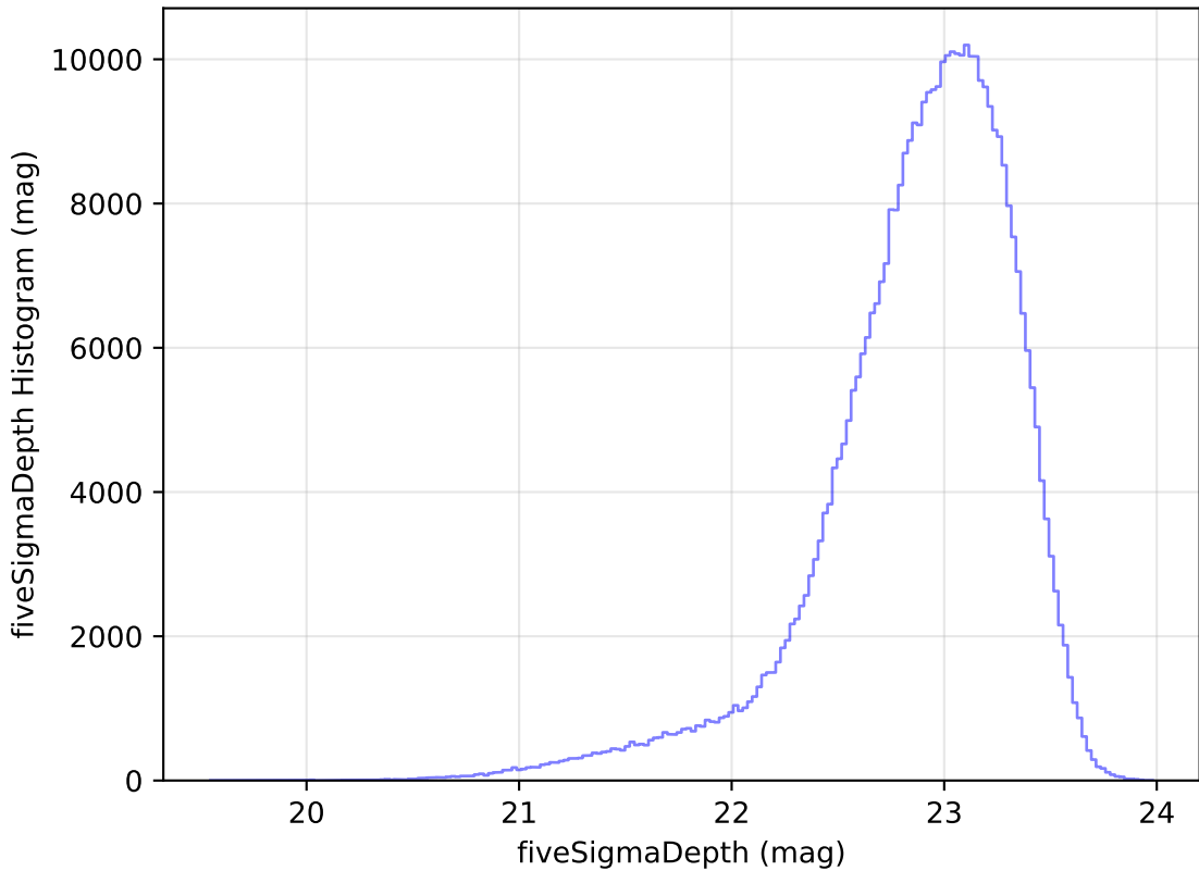
too_elab_r32_d3_giz_v3.4_10yrs WFD z band: fiveSigmaDepth Histogram
