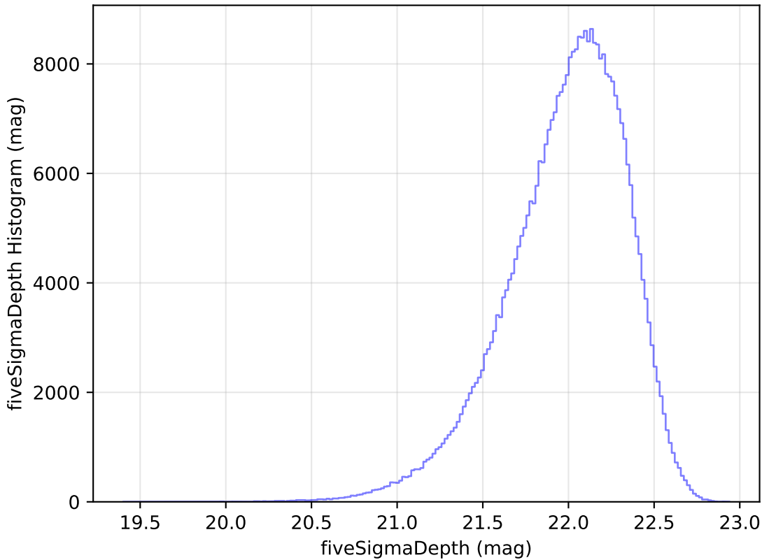
too_elab_r32_d3_giz_v3.4_10yrs WFD y band: fiveSigmaDepth Histogram
