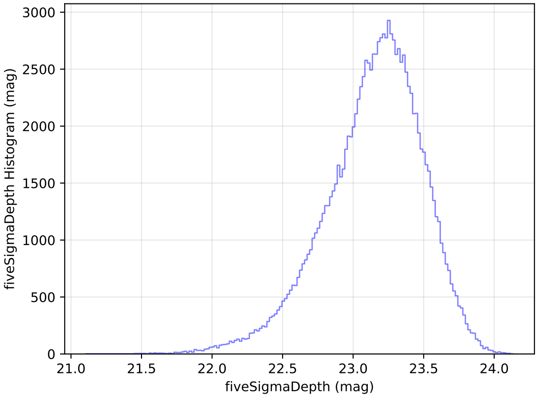
too_elab_r32_d3_giz_v3.4_10yrs WFD u band: fiveSigmaDepth Histogram
