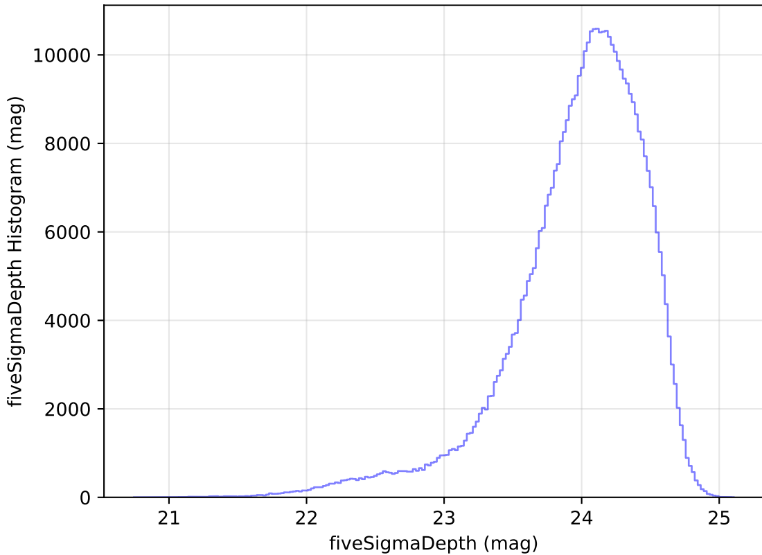
too_elab_r32_d3_giz_v3.4_10yrs WFD r band: fiveSigmaDepth Histogram
