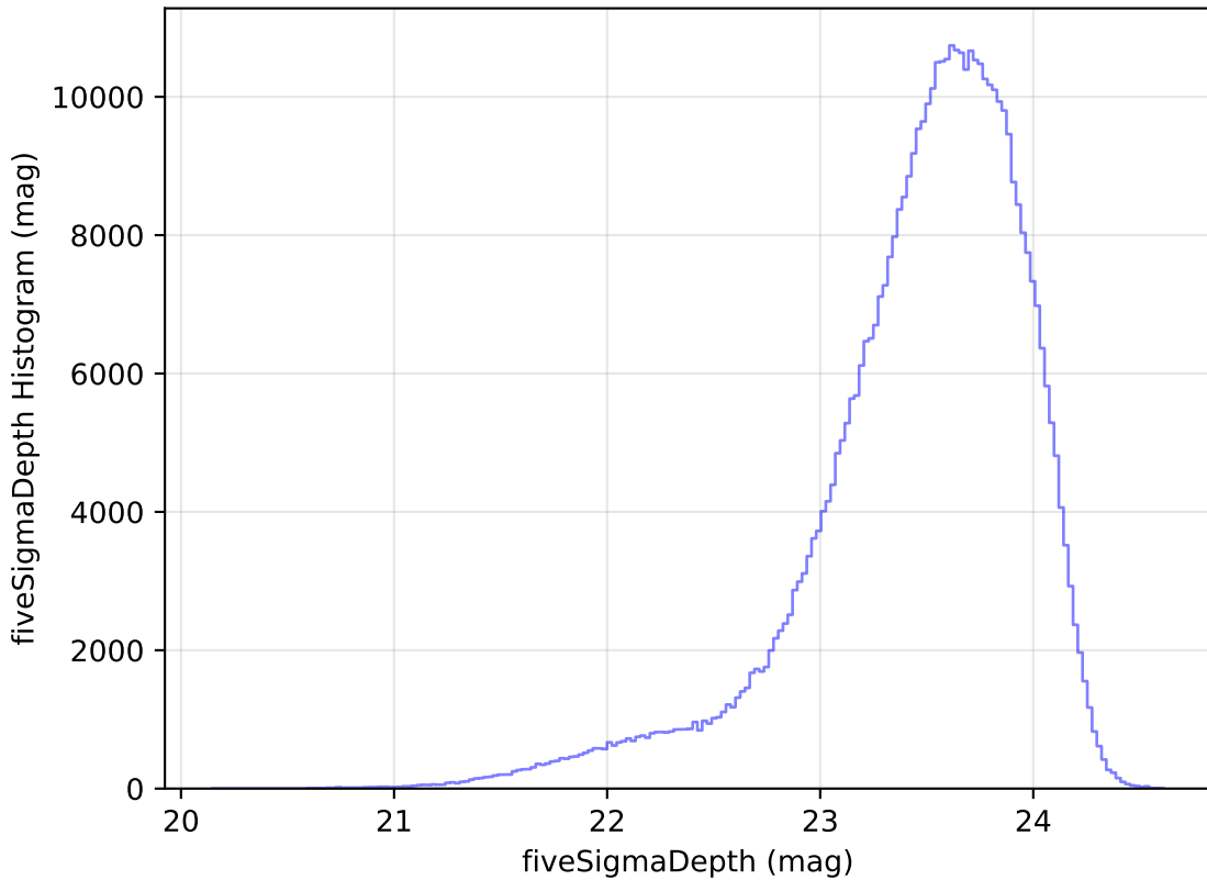
too_elab_r32_d3_giz_v3.4_10yrs WFD i band: fiveSigmaDepth Histogram
