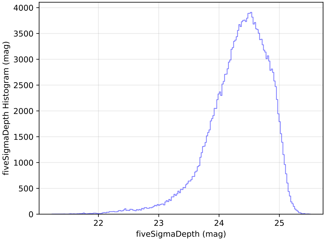
too_elab_r32_d3_giz_v3.4_10yrs WFD g band: fiveSigmaDepth Histogram
