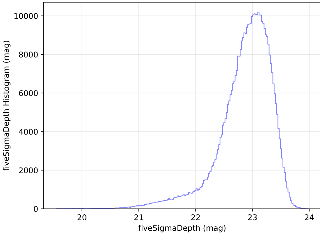
too_elab_r32_d3_giz_v3.4_10yrs All sky z band: fiveSigmaDepth Histogram
