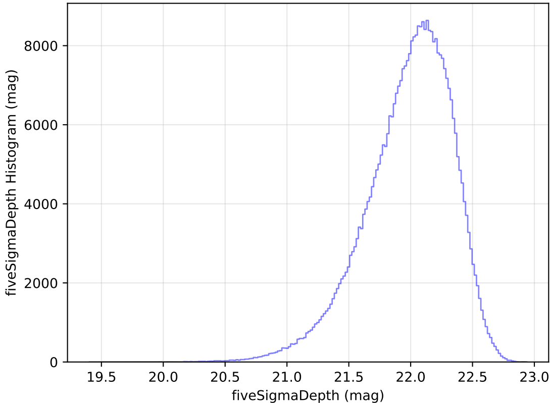
too_elab_r32_d3_giz_v3.4_10yrs All sky y band: fiveSigmaDepth Histogram
