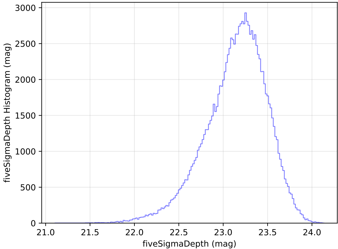
too_elab_r32_d3_giz_v3.4_10yrs All sky u band: fiveSigmaDepth Histogram
