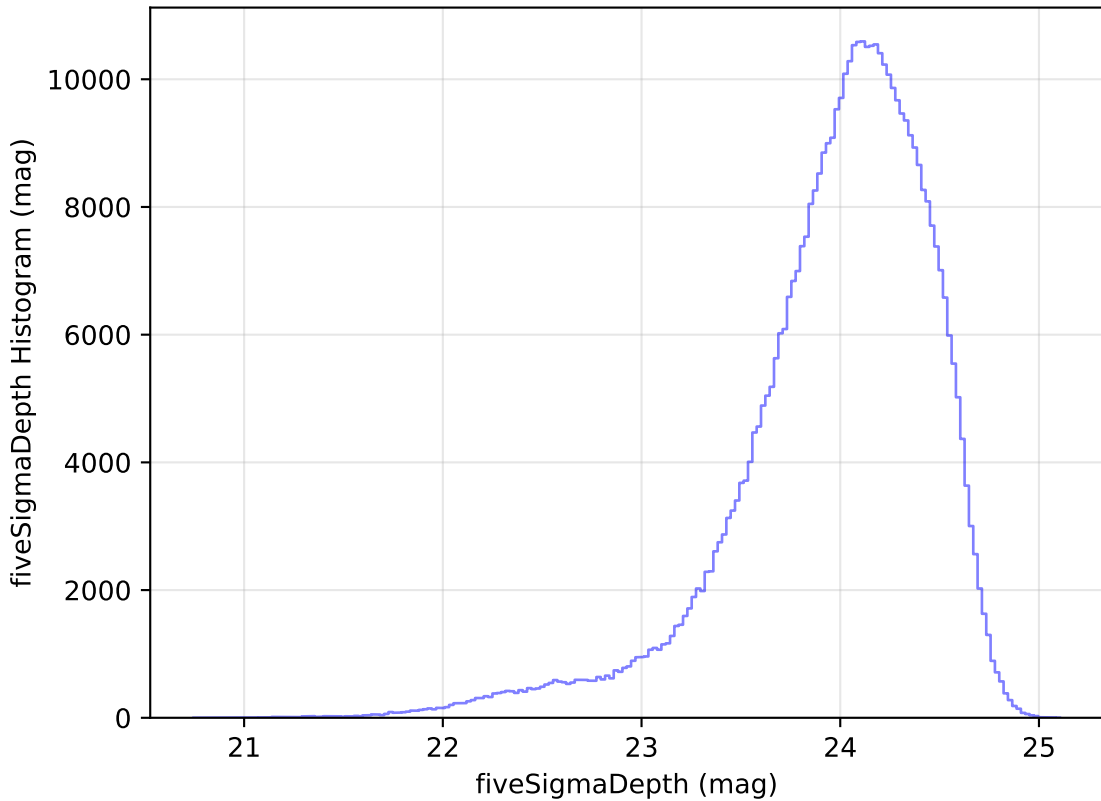
too_elab_r32_d3_giz_v3.4_10yrs All sky r band: fiveSigmaDepth Histogram
