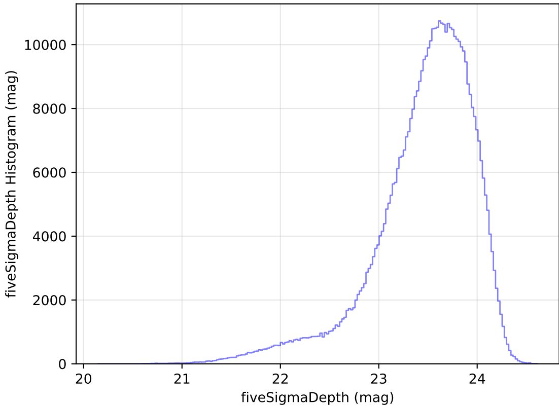
too_elab_r32_d3_giz_v3.4_10yrs All sky i band: fiveSigmaDepth Histogram
